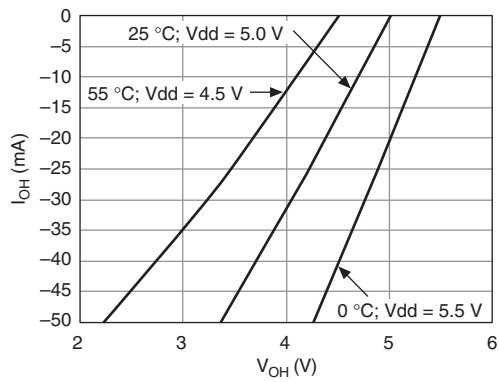
Figure 2. PFI <0..7>/P1: I_{OH} versus V_{OH}
