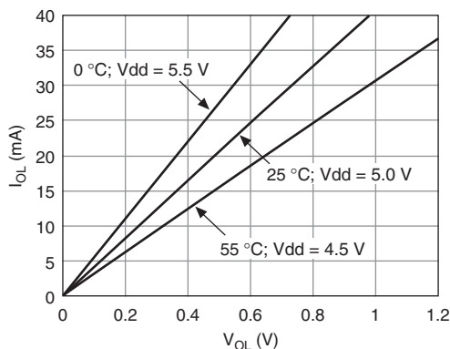
Figure 4. PFI <0..7>/P1: I_{OL} versus V_{OL}
